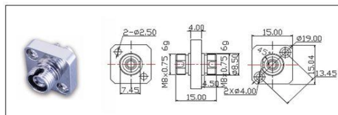
Figure1. FC Square Solid Body Adaptor
