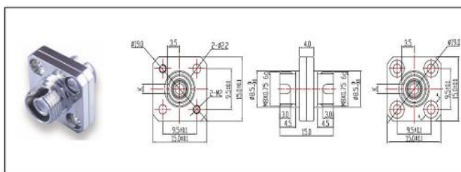
Figure2. FC Square Twain Adaptor
