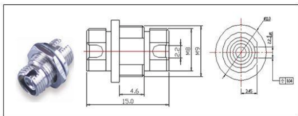
Figure5. FC D3 Adaptor
