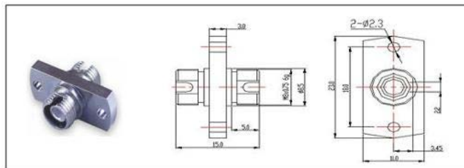
Figure3. FC Rectangle Adaptor
