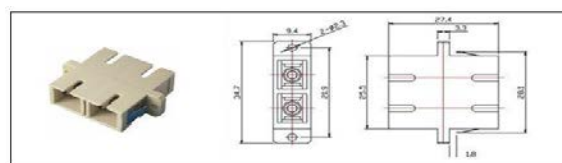
Figure3. SC Duplex Adapter
