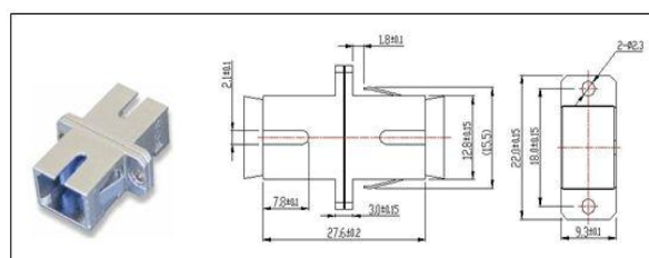
Figure2. SC Simplex Metal Adapter
