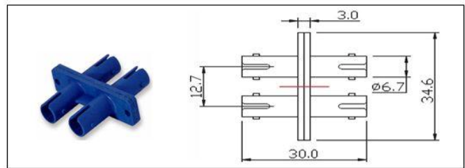
Figure2. ST SC Footprint Duplex Plastic Adaptor
