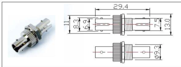
Figure1. ST D-Shaped Adaptor
