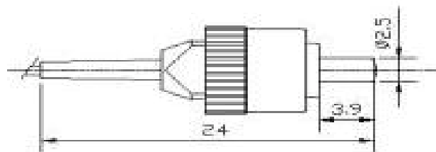
Figure 2 : FC 0.9 Connector
