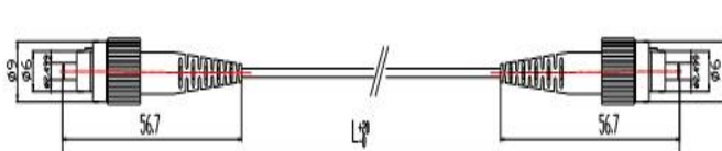
Figure2: FC-FC Patchcord 2.0/3.0mm
