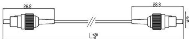
Figure1: FC-FC Patchcord 0.9mm
