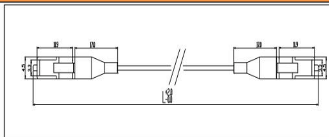
Figure1. LC 0.9 Patch Cord
