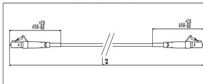
Figure2. LC 2.0 Patch Cord
