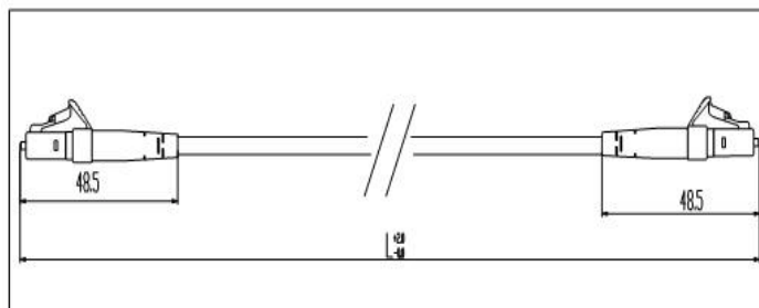
Figure3. LC 3.0 Patch Cord
