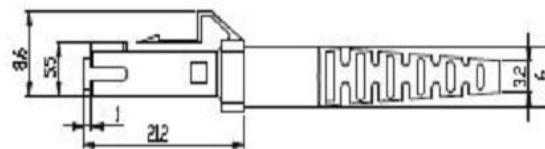
Figure2: MTRJ 3.0 Connector
