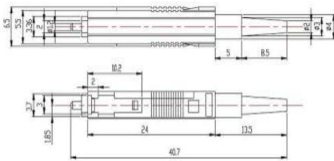
Figure1: MU 0.9 Connector
