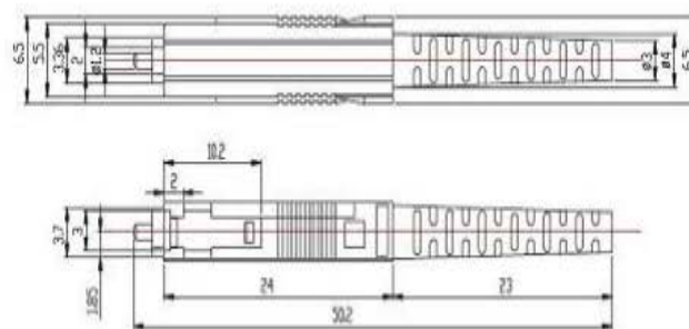
Figure2: MU 2.0/3.0 Connector
