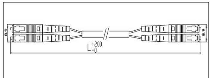
Figure2. MU 2.0 Patch Cord
