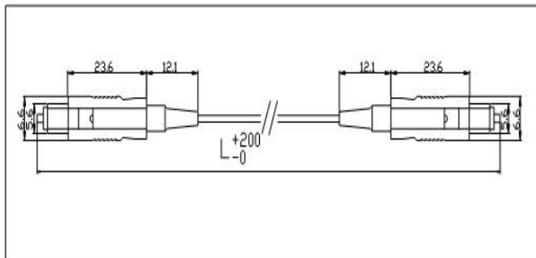
Figure1. MU 0.9 Patch Cord
