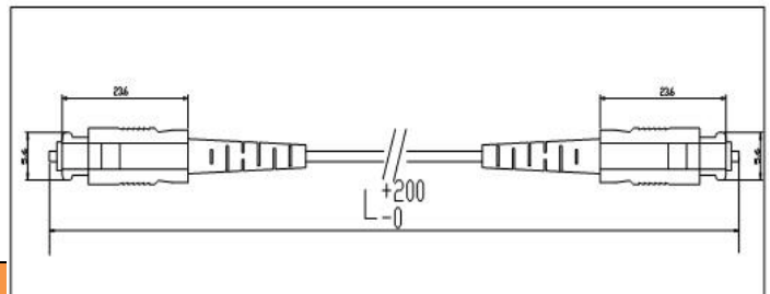
Figure2. MU 2.0 Patch Cord
