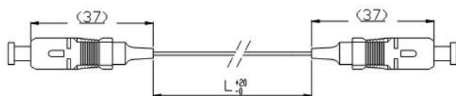
Figure1: SC-SC Patchcord 0.9mm
