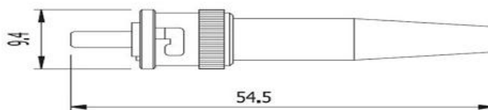
Figure2: ST 3.0/2.0 Connector
