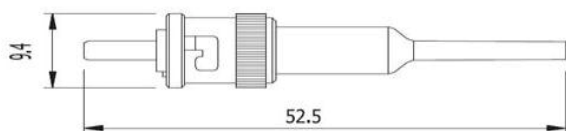
Figure1: ST 0.9 Connector
