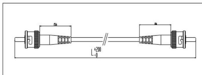
Figure2. ST 2.0/3.0 Patch Cord Appearance
